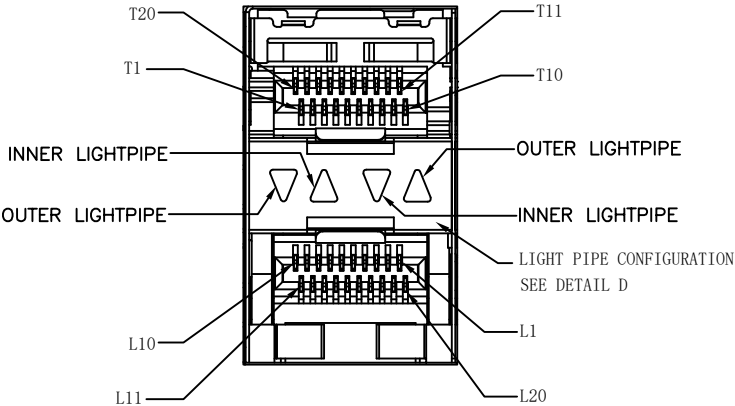
DETAIL C SCALE 4:1
